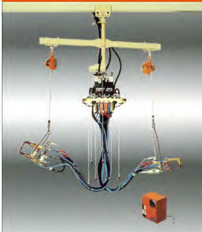
PORTABLE SPOT WELDING SYSTEM (PORTABLE SPOT WELDING GUN, TRANSFORMER, TIMER CONTROLLER)
